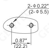
Rear Bracket Mounting
